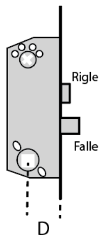
Cylinder: Oval
